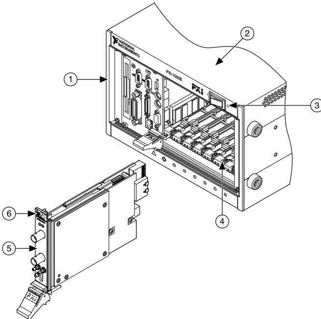
Figure 3. Module Installation
