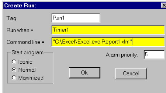
Figure 18-105. Run Definition Parameters Dialog Box
