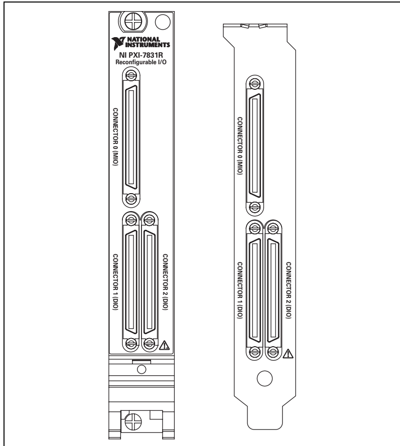
Figure 1. NI 7831R Connector Locations
