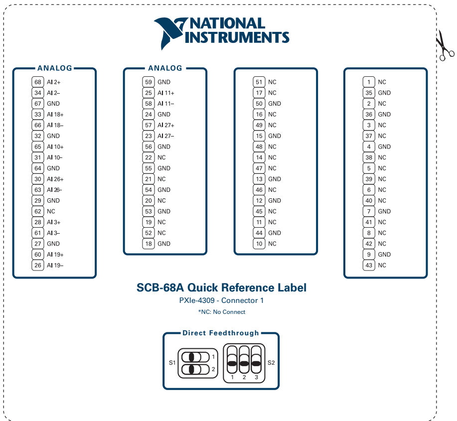
Figure 2. PXIe-4309 Connector 1
