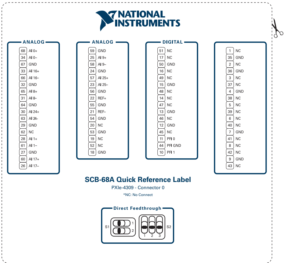
Figure 1. PXIe-4309 Connector 0
