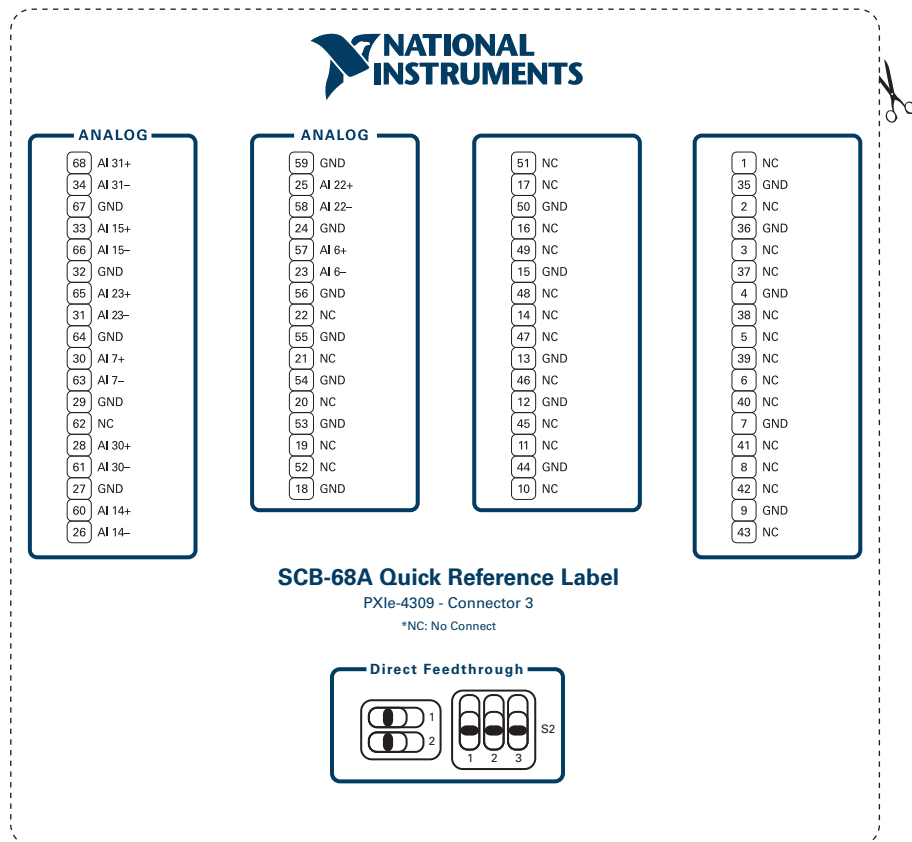
Figure 4. PXIe-4309 Connector 3
