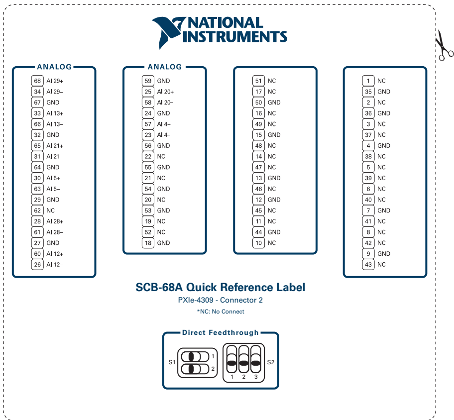
Figure 3. PXIe-4309 Connector 2
