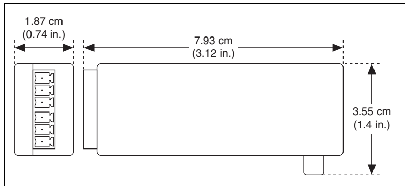
Figure 3. SCC-RTD01 Dimensions
