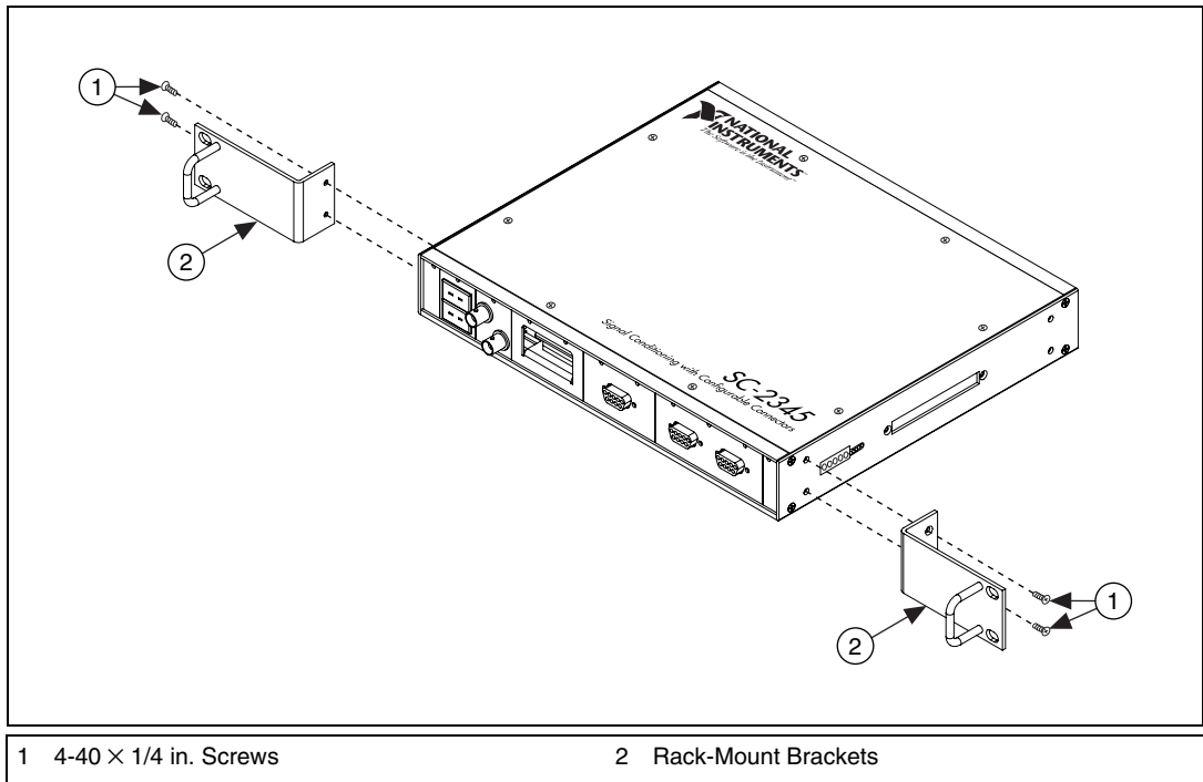
Figure 2-2. Rack-Mount Option
