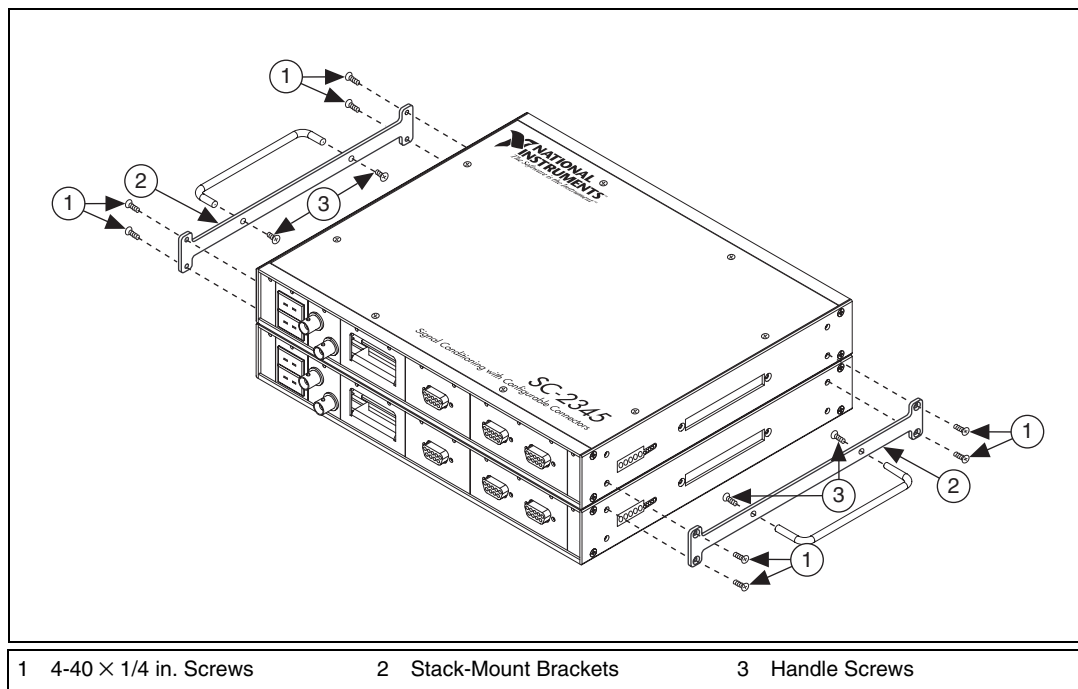
Figure 2-3. Stack-Mount Option
