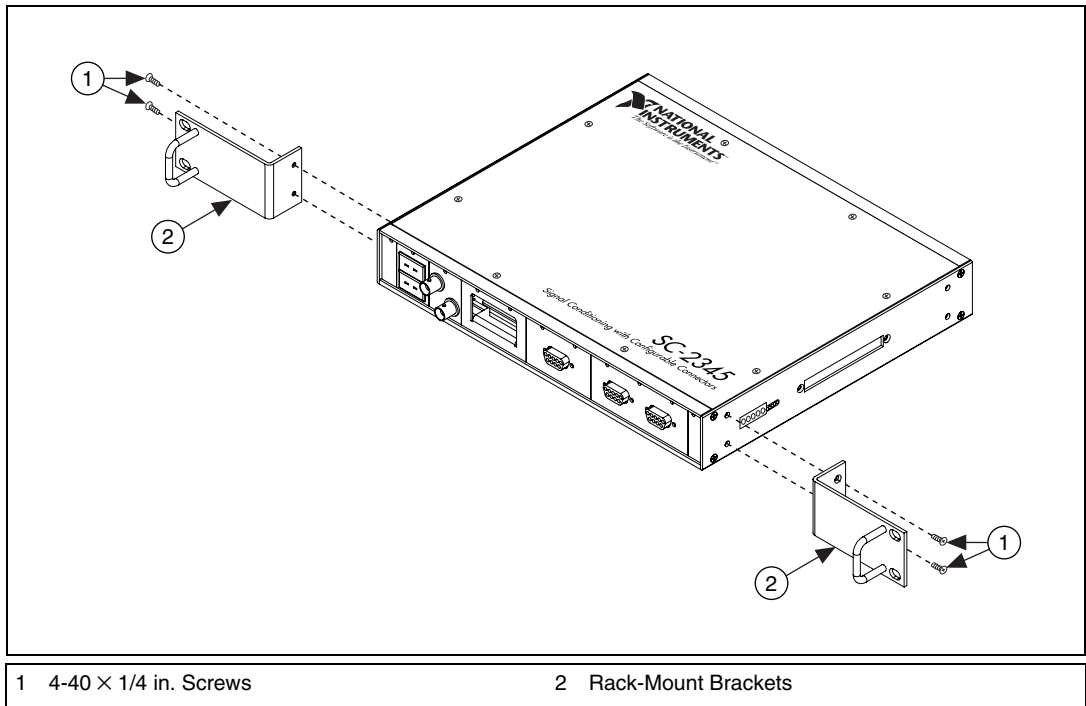
Figure 2-2. Rack-Mount Option
