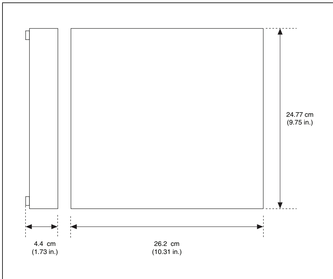
Figure A-1. SC-2345 Connector Block Dimensions
