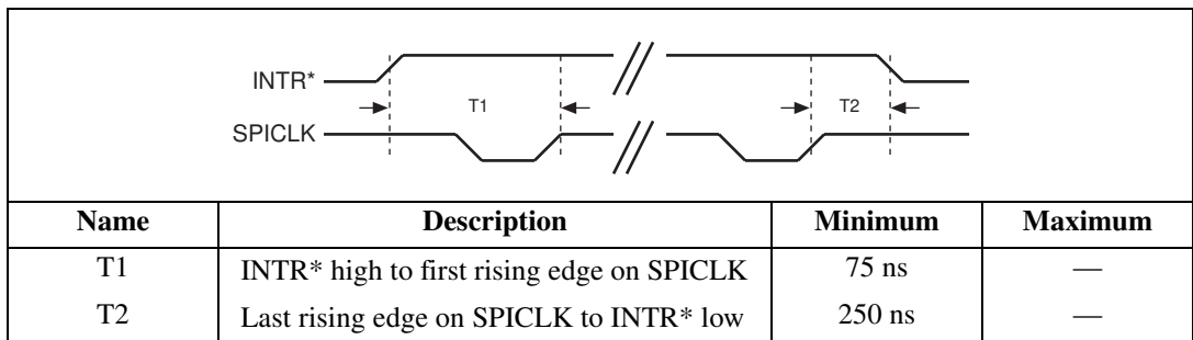
Figure 5. Slot 0 Register Writes Diagram
