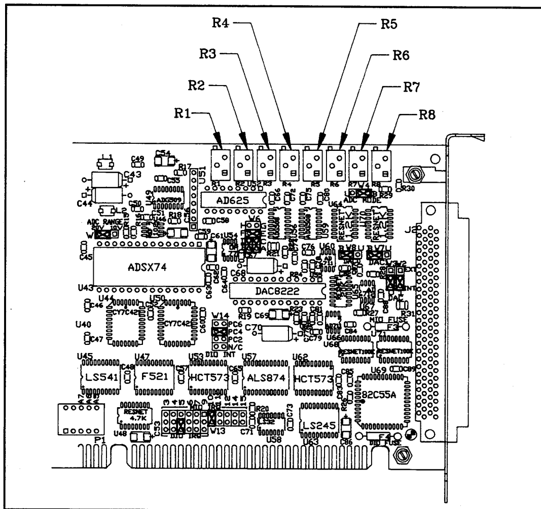
Figure 5-1. Calibration Trimpot Location Diagram
