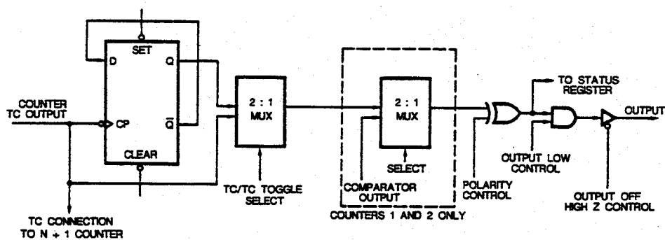
Figure 17. Output Control Logic
