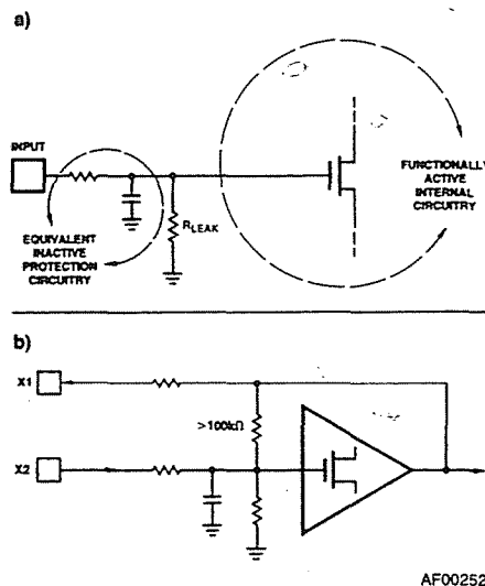
Figure 1-4. Input Circuitry
