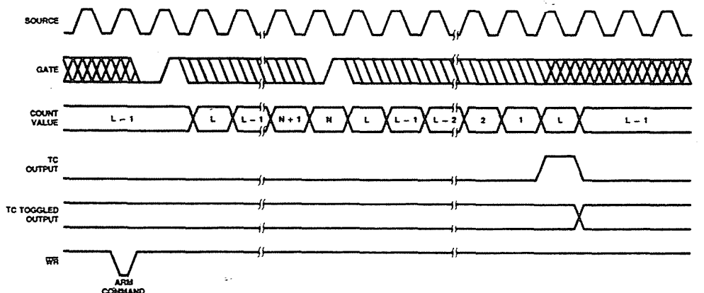
Figure 1-16o. Mode O Waveforms
