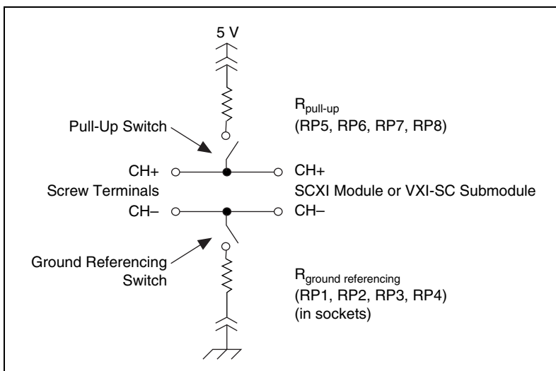
Figure 5. Resistor Connections
