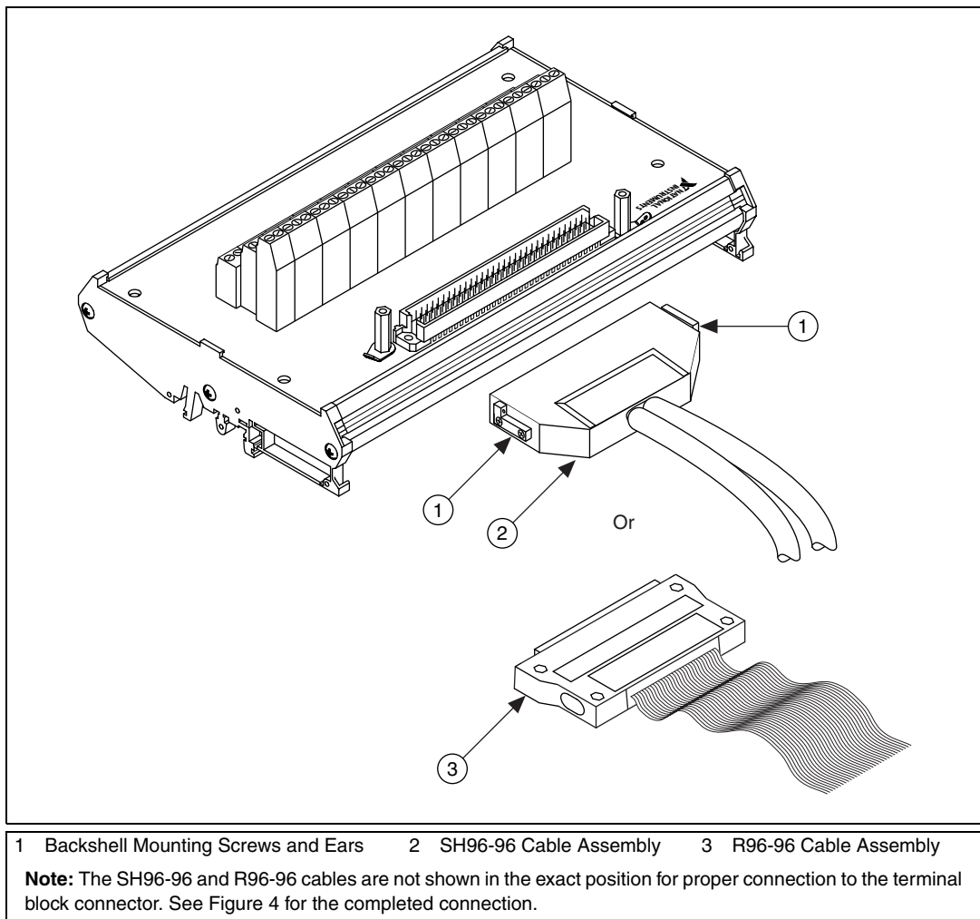
Figure 3. Connecting the SH96-96 or R96-96 Cable to the TBX-96 Terminal Block
