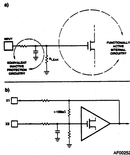
Figure 3. Input Circuitry
