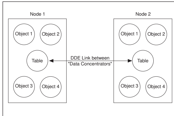
Figure 14-2. Table Networking
