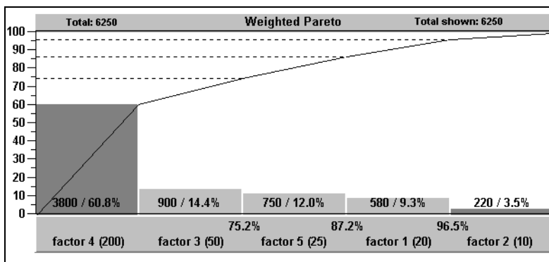
Figure 18-88. Weighted Pareto Chart
