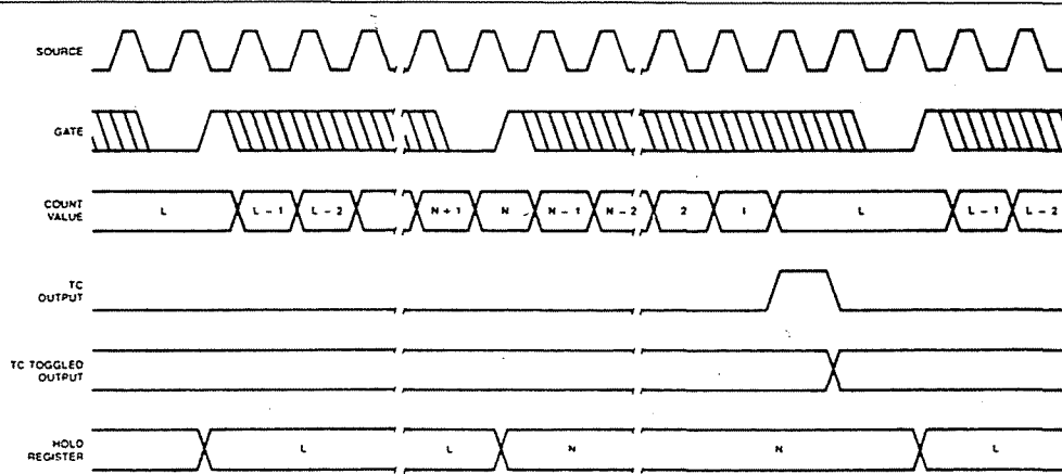
Figure 1-16x. Mode X Waveforms
