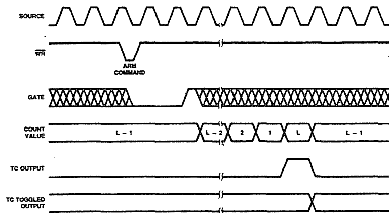
Figure 1-16c. Mode C Waveforms
