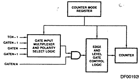
Figure 1-13. Gating Control
