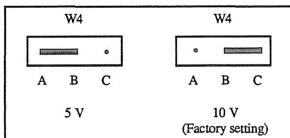
Figure 2-9. Reference Choice Configurations
