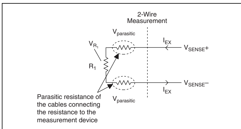
Figure 2-8. Signal Connections for a 2-Wire Resistance Measurement
