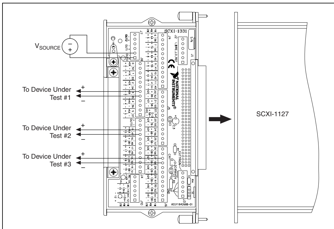
Figure 2-18. 1 \times 32 Matrix Wiring Diagram
