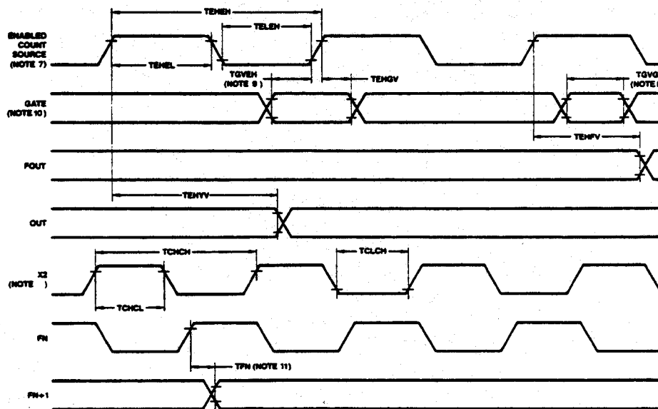
Figure 22. Counter Switching Waveforms
