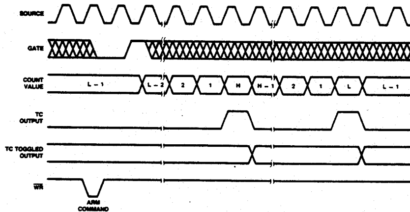
Figure 15i. Mode I Waveforms
