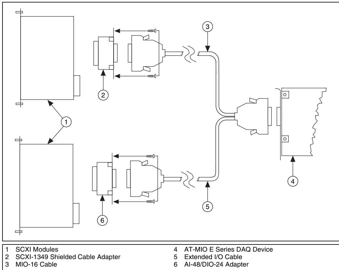
Figure 1. SCXI-1353 Installation
