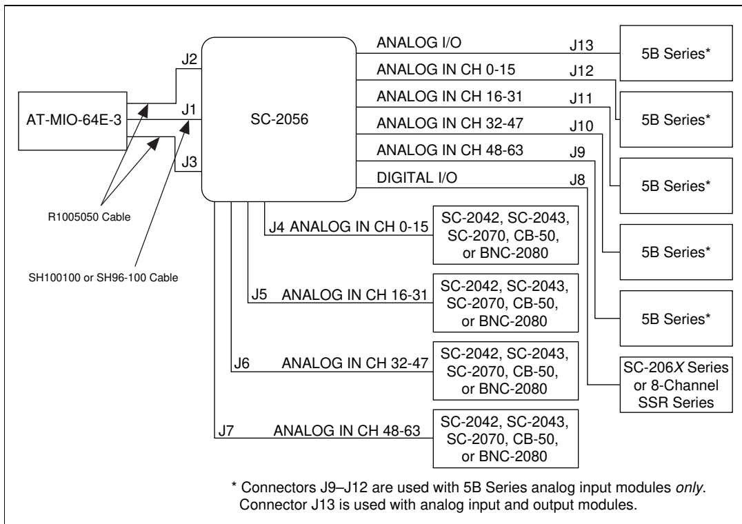
Figure 8-2. SC-2056 Connections
