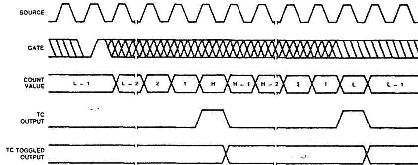
Figure 1-16l. Mode L Waveforms
