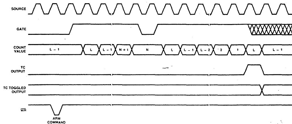
Figure 1-16n. Mode N Waveforms
