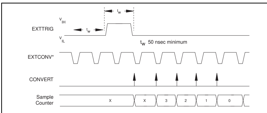
Figure 2-11. Posttrigger DAQ Timing (EXTCONV* High When Trigger Sensued)
