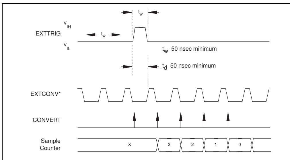
Figure 2-12. Posttrigger DAQ Timing (EXTCONV* Low When Trigger Sensued)
