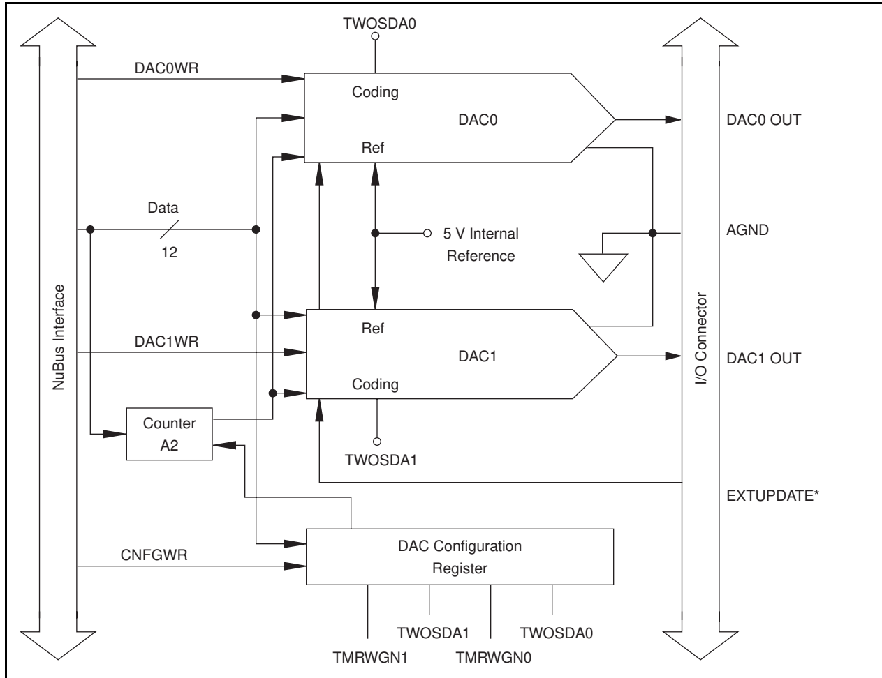
Figure 3-4. Analog Output Circuitry Block Diagram
