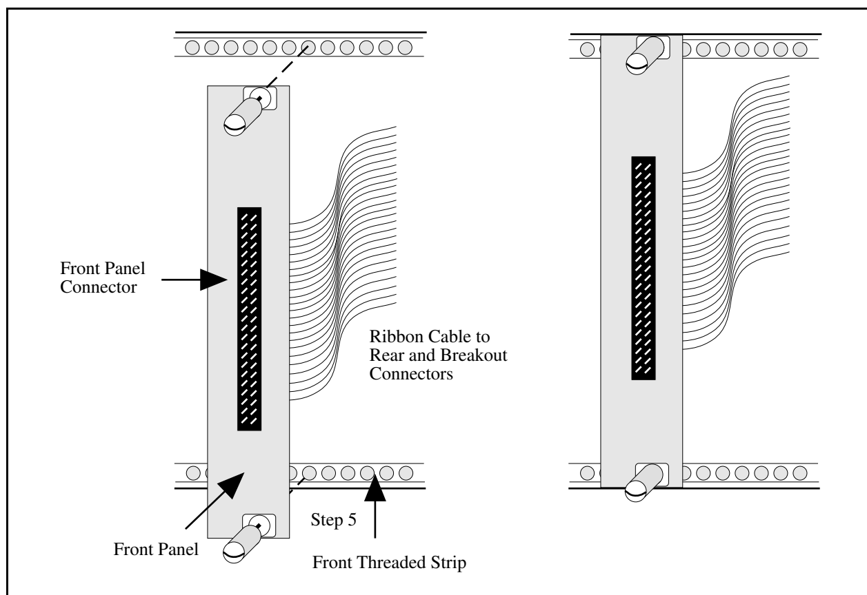
Figure 2-5. SCXI-1180 Front Panel Installation
