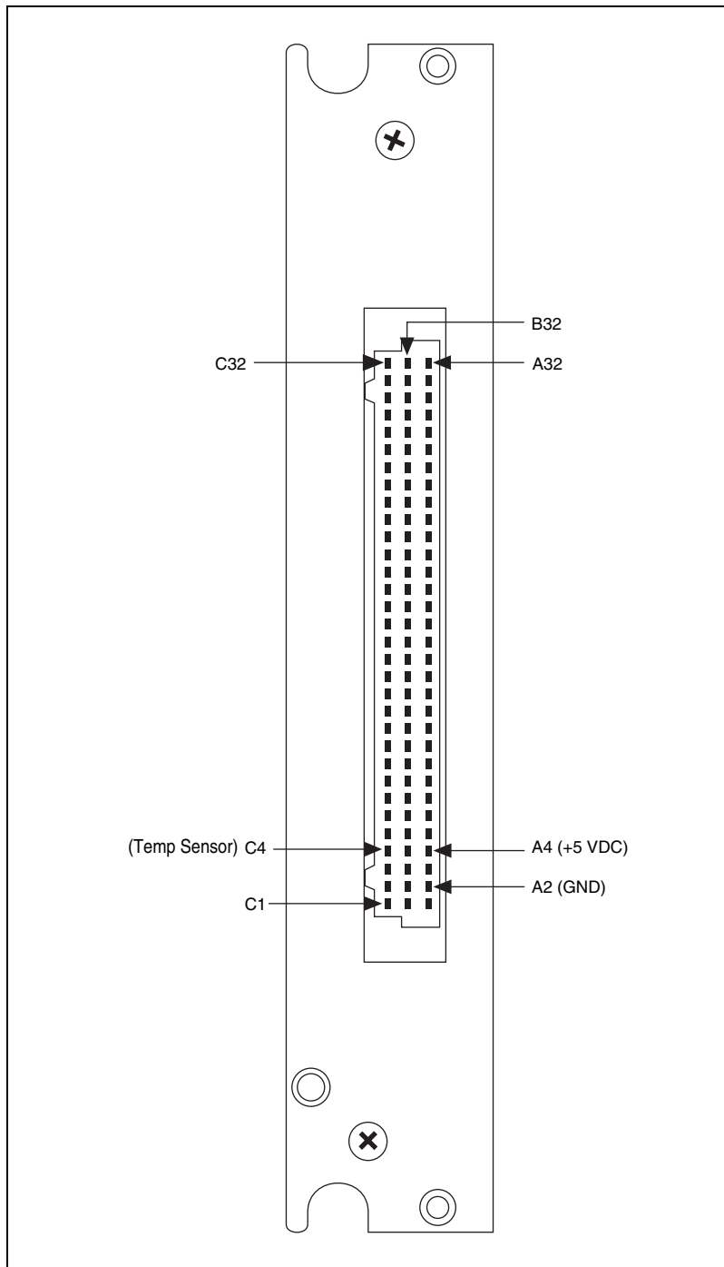
Figure 3. SCXI-1313 Connector Pin Assignments
