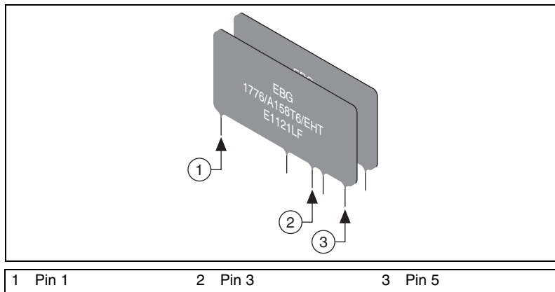
Figure 1. SCXI-1313A Resistor Network Pin Designations
