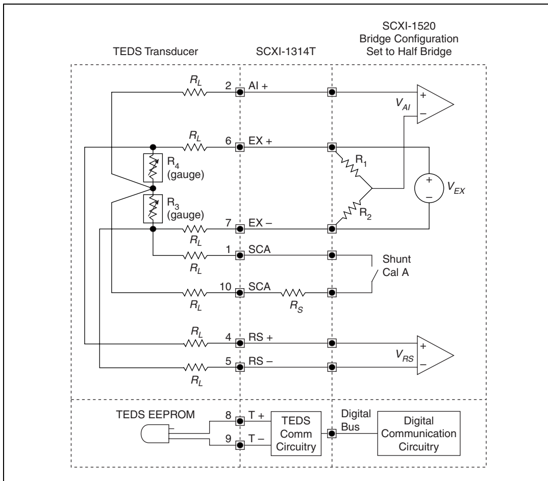
Figure 4. Half-Bridge Circuit Diagram
