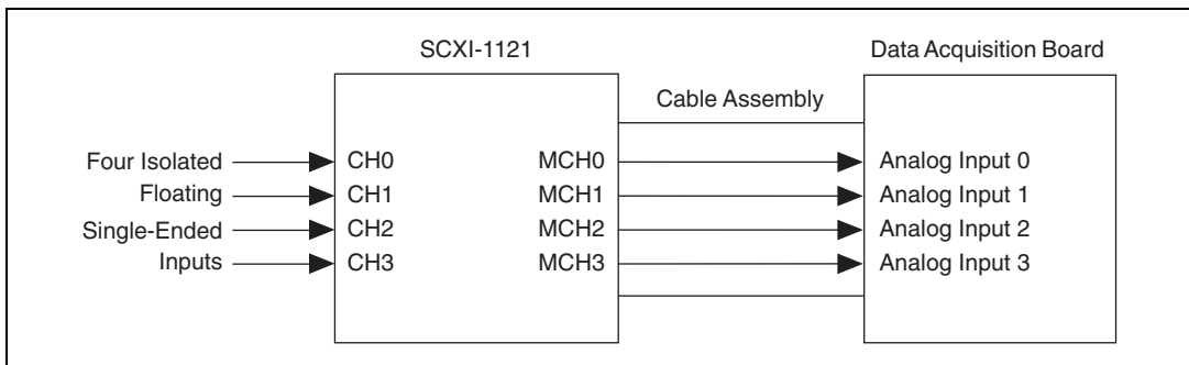
Figure 3-7. Single-Module Parallel Scanning
