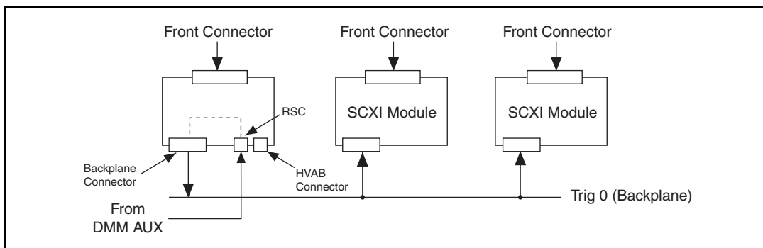
Figure 2-12. Cabling a DMM and Using the TRIG0 to Bus the VMC/EXT_TRIG_IN to Non-Cabled Modules
