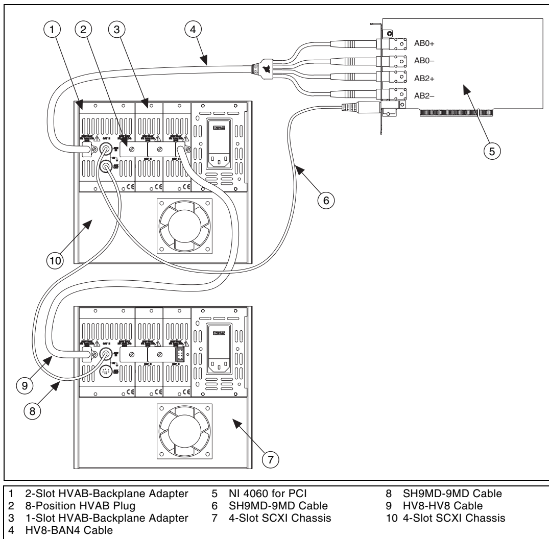
Figure 1-6. 4-Slot to 4-Slot Multichassis Configuration Parts Locator Diagram
