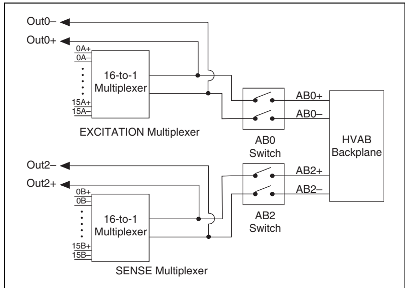
Figure 2-6. 4-Wire Block Diagram
