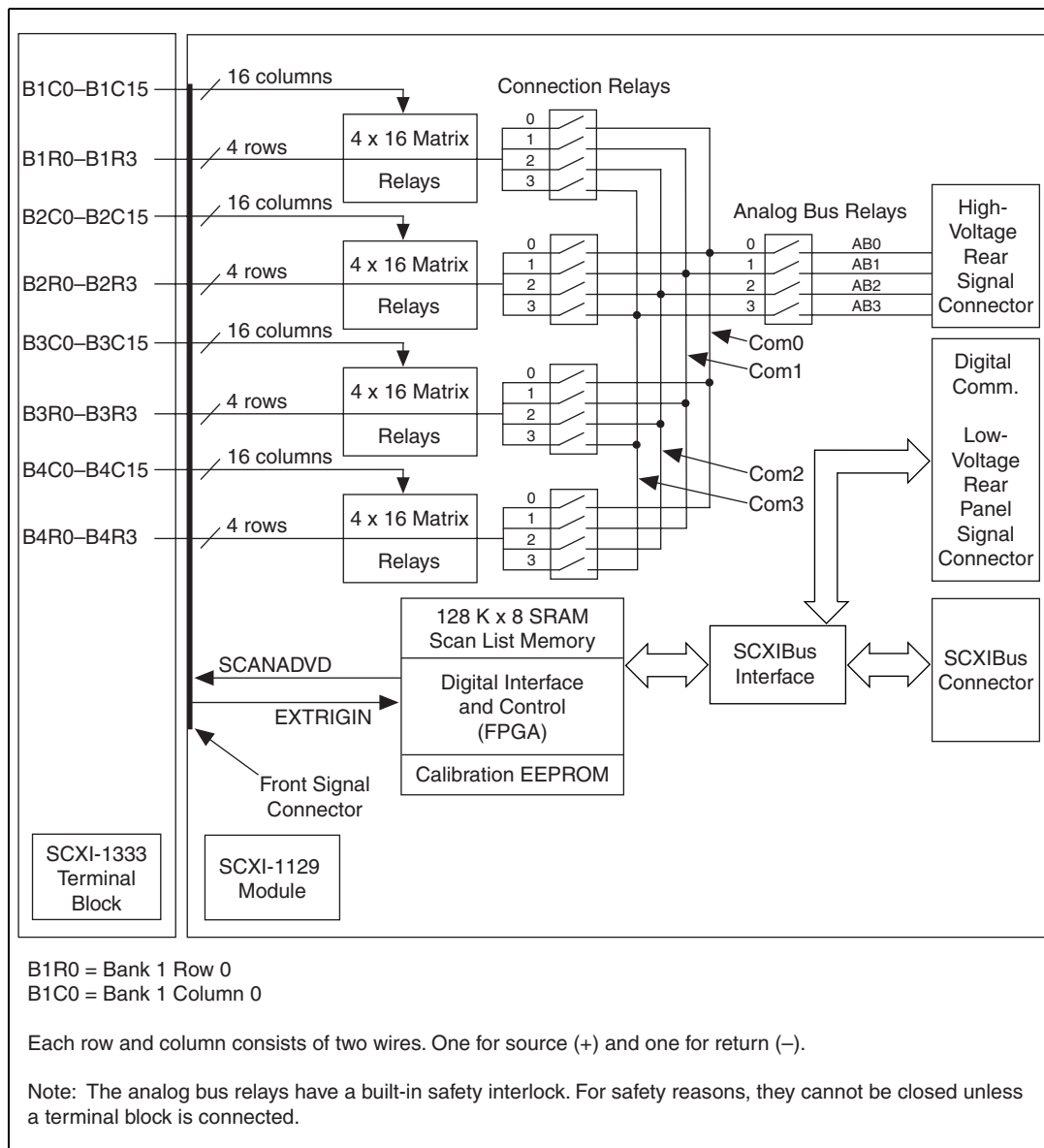
Figure 2-4. 4 \times 16 Matrix Configuration
