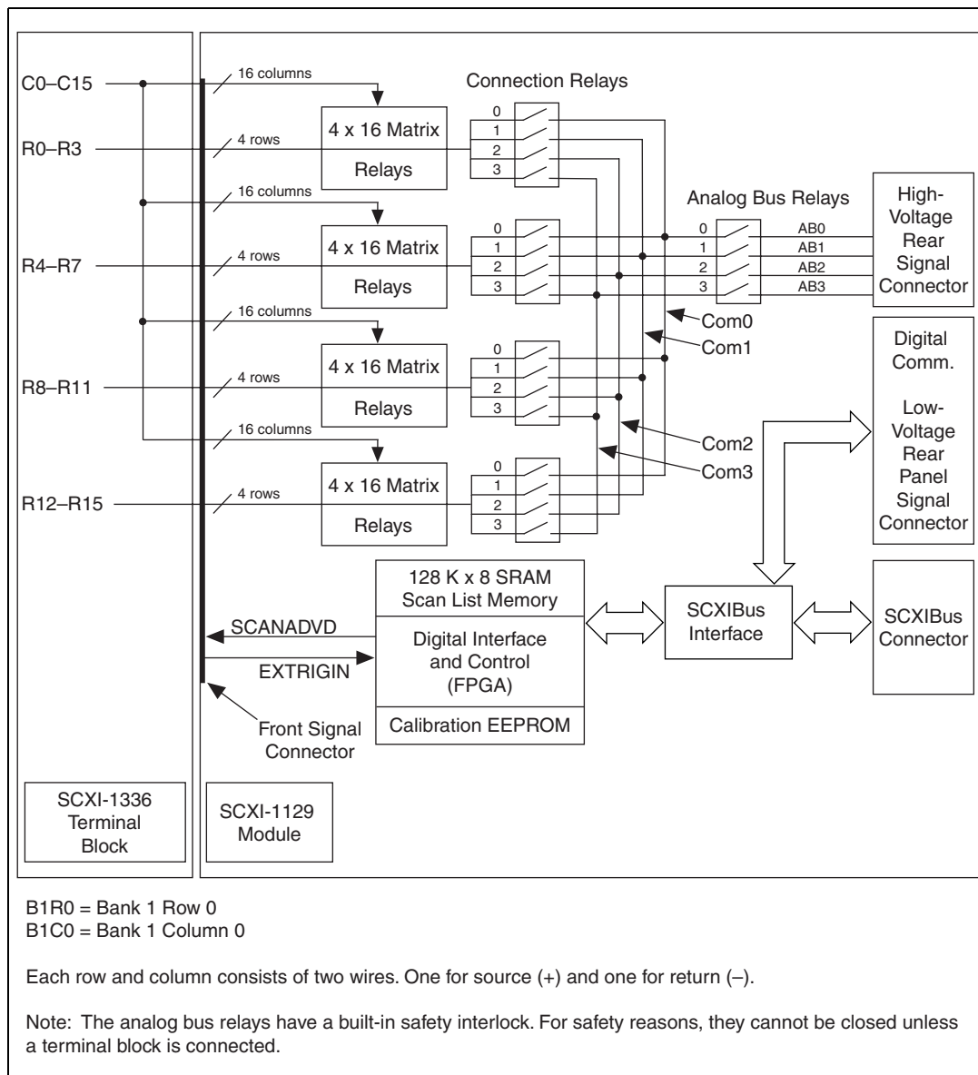
Figure 2-10. 16 × 16 Matrix Configuration
