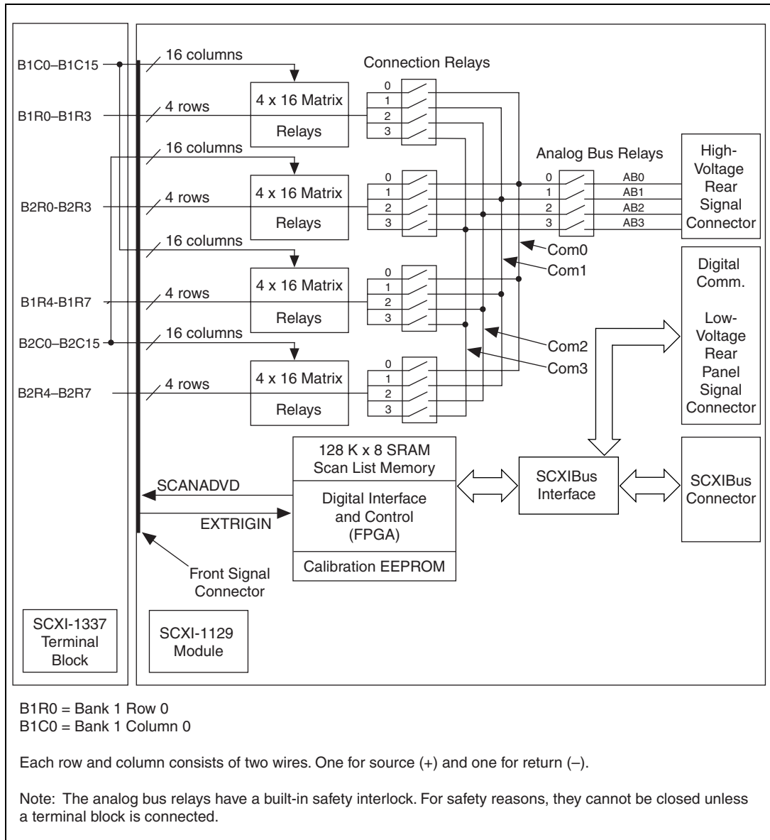
Figure 2-6. 8 \times 16 Matrix Configuration
