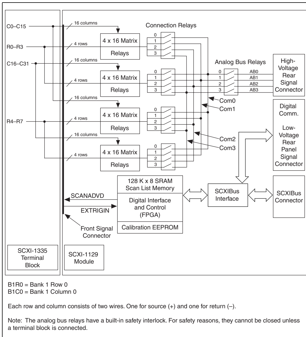
Figure 2-8. 8 x 32 Matrix Configuration
