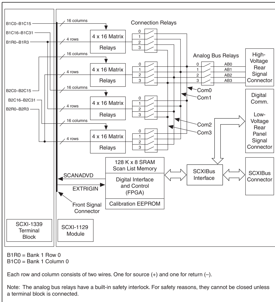
Figure 2-5. 4 × 32 Matrix Configuration
