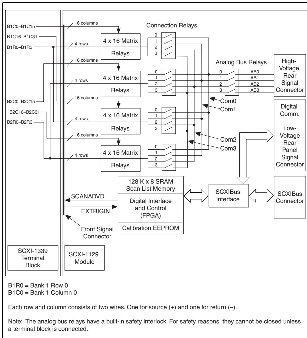
Figure 2-5. 4 \times 32 Matrix Configuration
