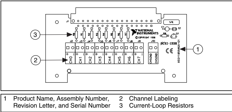
Figure 1. SCXI-1338 Signal Connections
