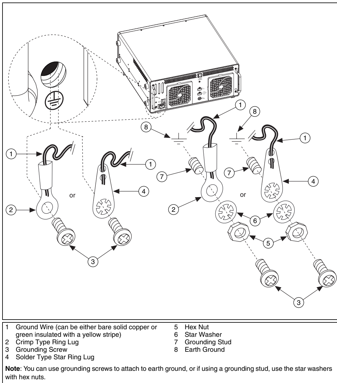
Figure 2-1. Grounding the PXI-1011 Chassis
