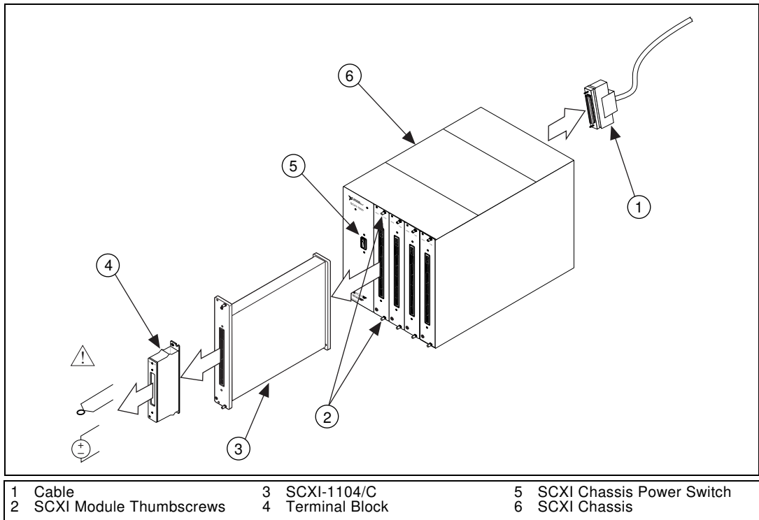
Figure 2-3. Removing the SCXI-1104/C
