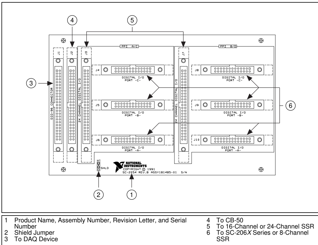
Figure 6-1. SC-2054 Parts Locator Diagram
