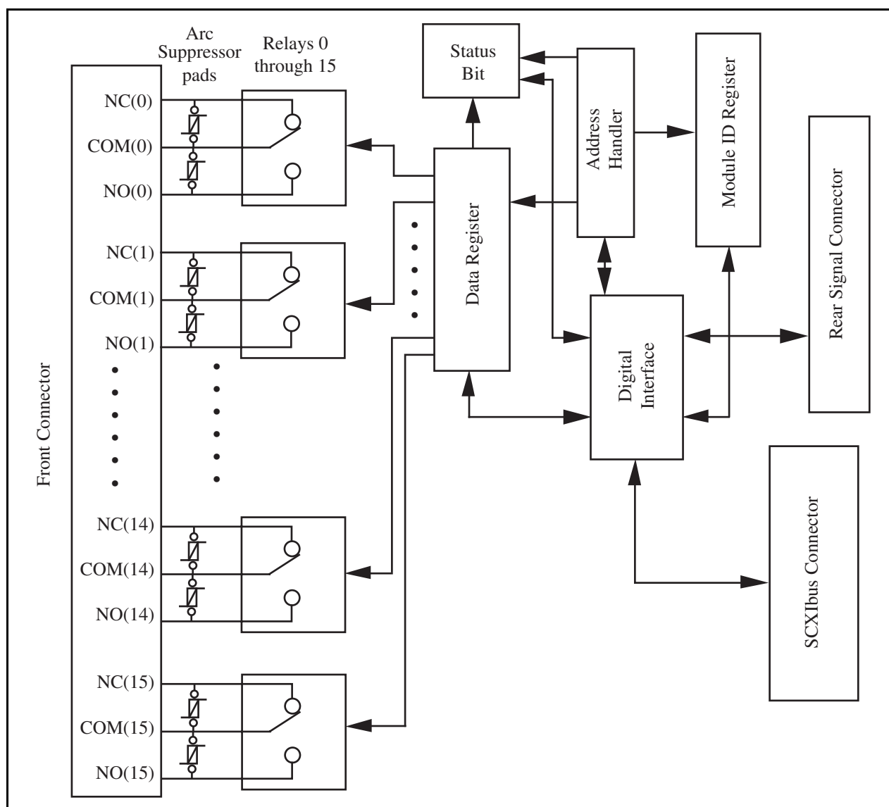
Figure 3-1. SCXI-1160 Block Diagram
