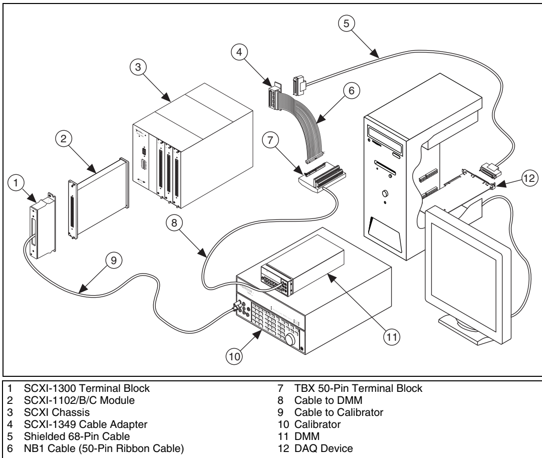
Figure 1. Calibration Connections
