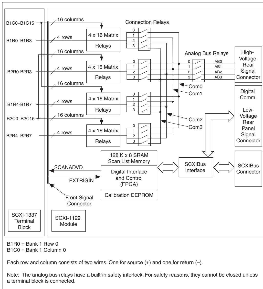
Figure 2-6. 8 x 16 Matrix Configuration
