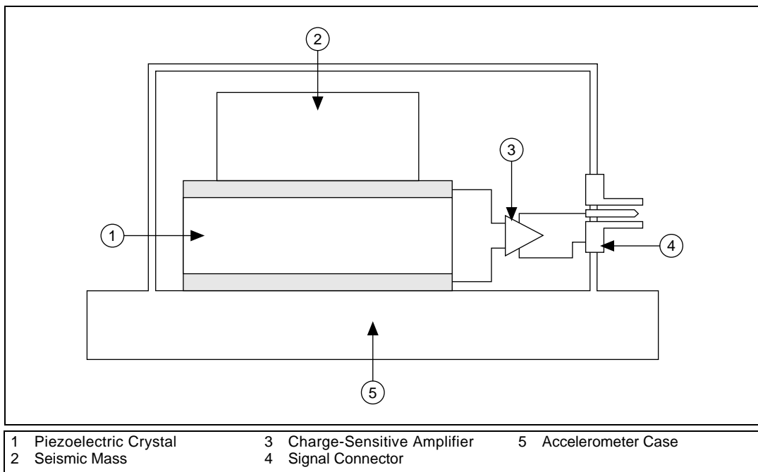
Figure 2-1. Typical Current-Excited Accelerometer
