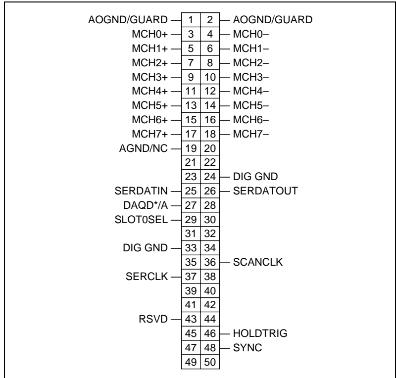
Figure 2-4. SCXI-1530/1531 Rear Signal Connector
