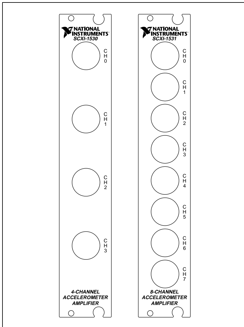
Figure 2-3. SCXI-1530/1531 BNC Connector Assignments
