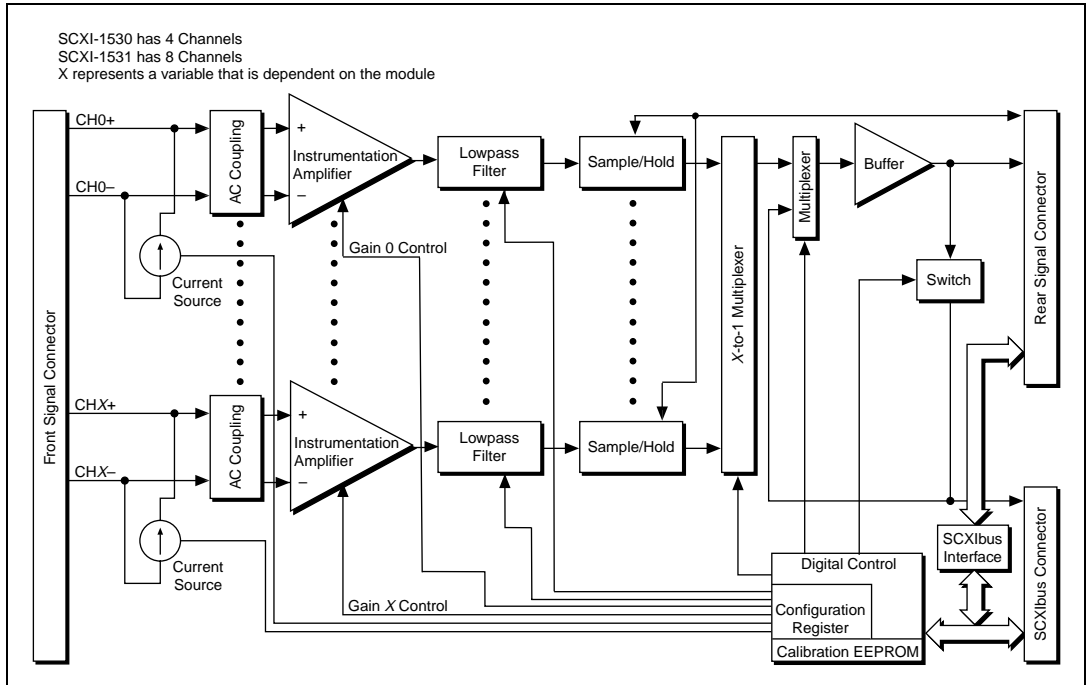
Figure 2-2. SCXI-1530/1531 Module Block Diagram
