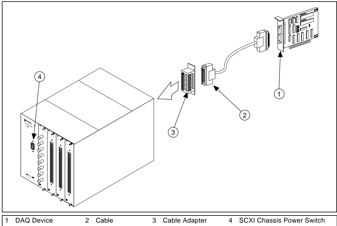
Figure 1-2. Connecting an SCXI Chassis to a DAQ Device
