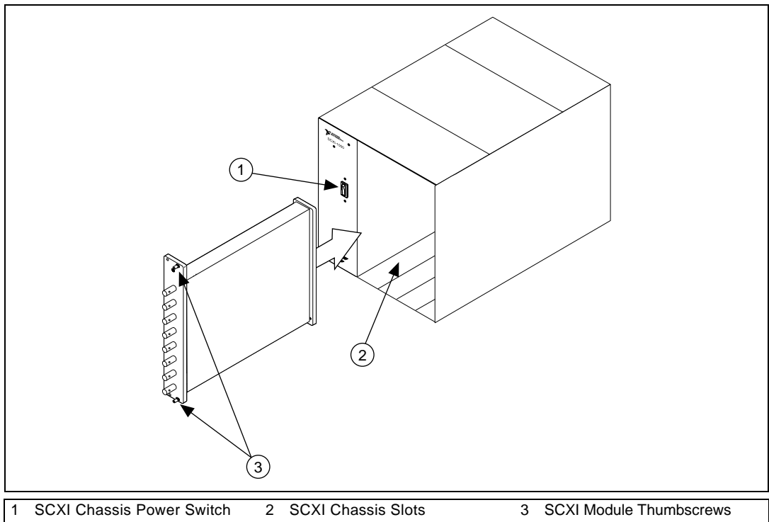
Figure 1-1. Installing the SCXI-1530/1531 Module
