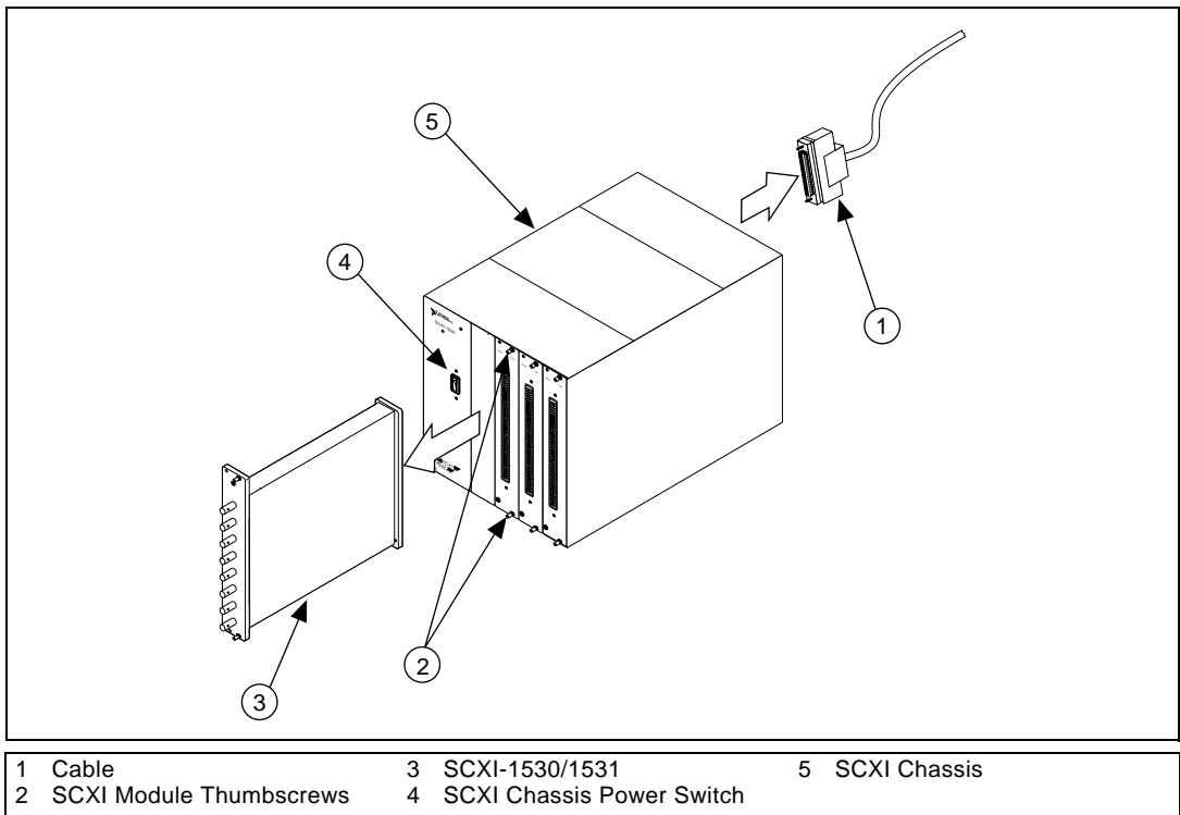
Figure 1-3. Removing the SCXI-1530/1531
