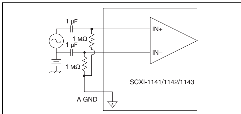
Figure 2-4. Ground Offset AC-Coupled Signal Connection
