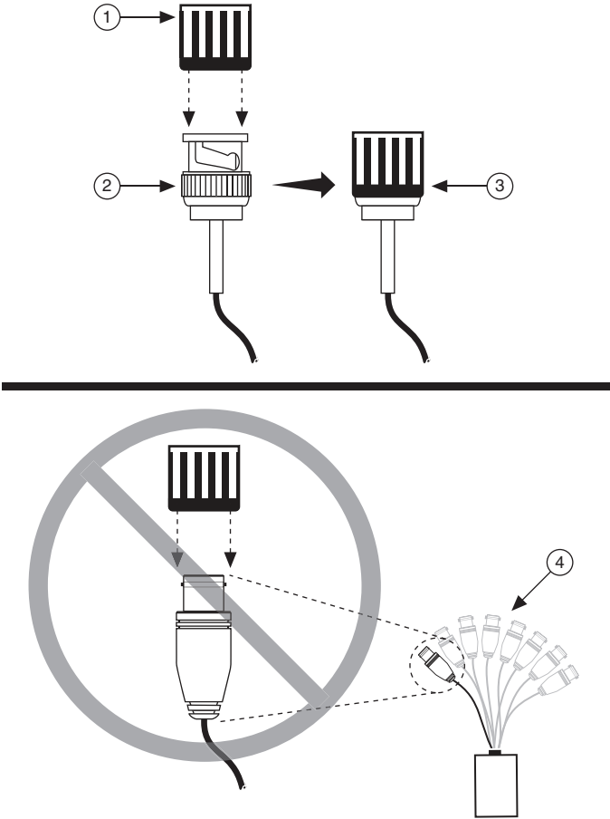
Figure 1. Coaxial Connector Cover Installation
