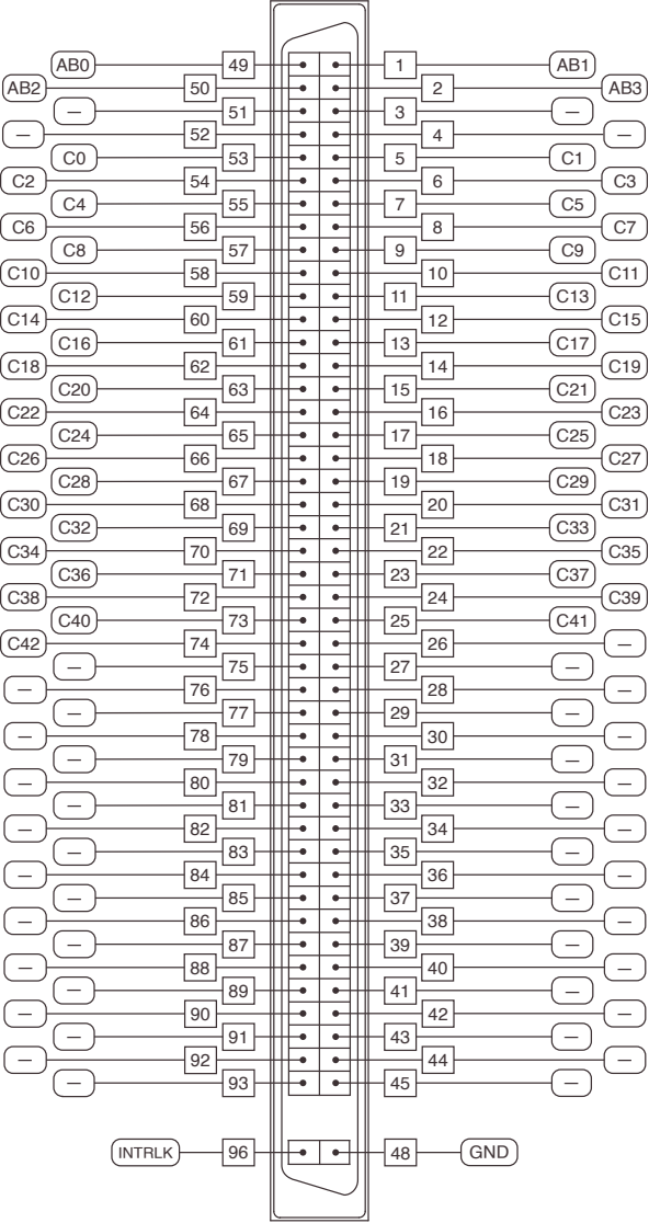
Figure 1. SWB-2810A/B Connector Pinout
