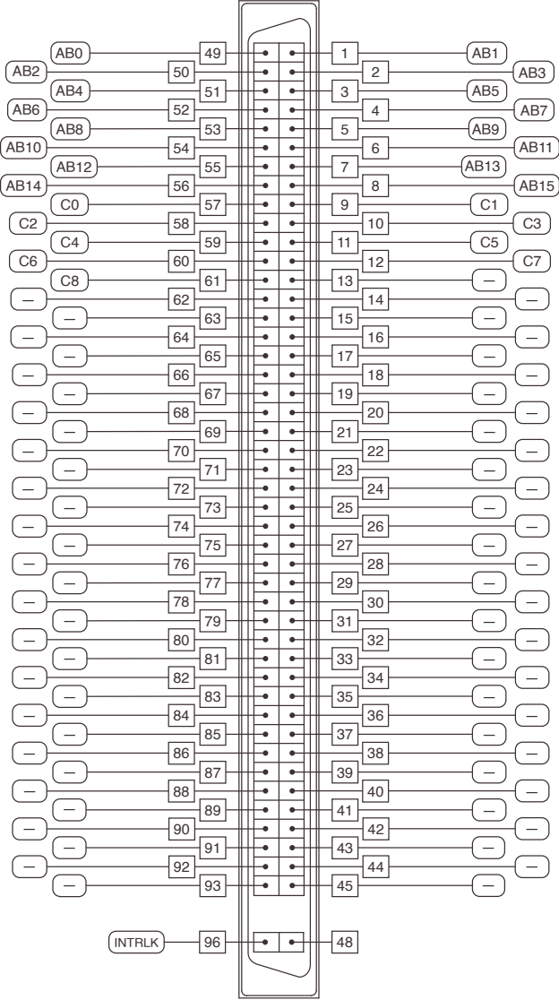
Figure 1. SWB-2812 Connector Pinout
