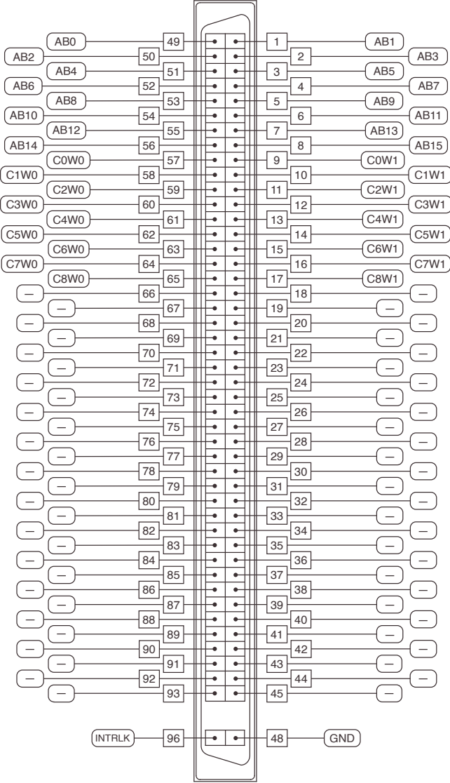
Figure 1. SWB-2814 Connector Pinout
