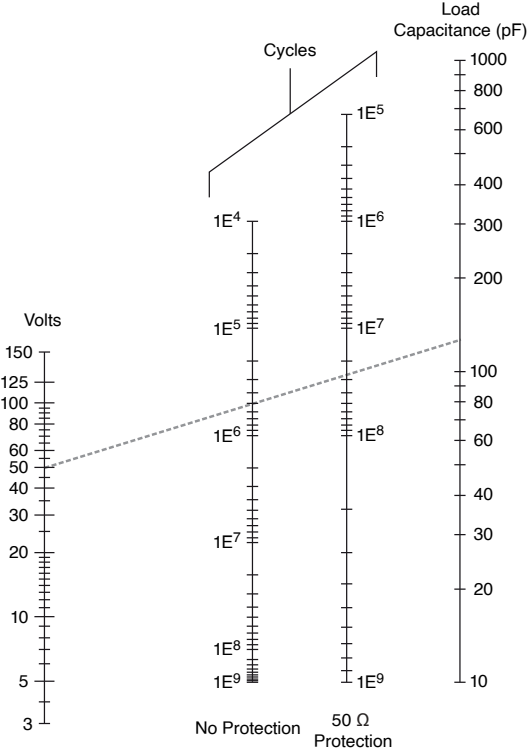
Figure 3. Reed Relay Life Nomograph Solution
