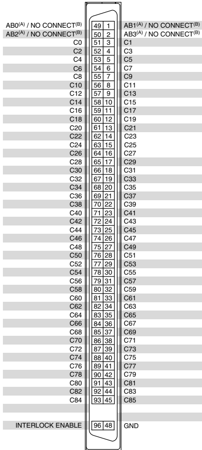
Figure 2. NI 2815A/B Connector Pinout
