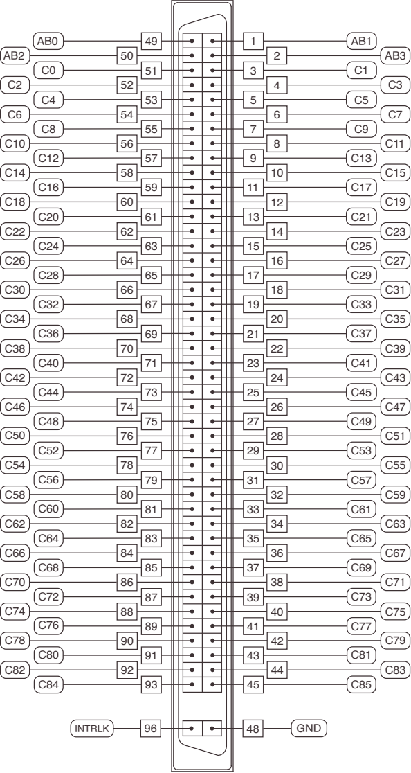
Figure 1. SWB-2815 Connector Pinout
