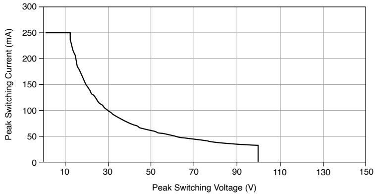
Figure 2. Peak Switching Voltage Versus Current
