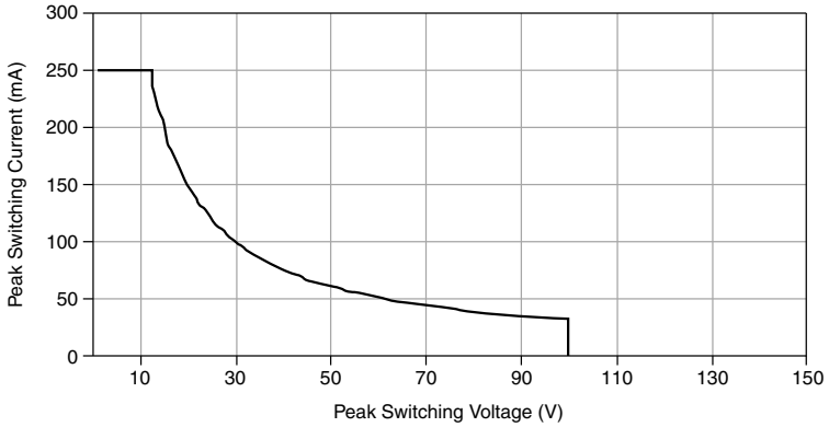
Figure 1. Peak Switching Voltage Versus Current
