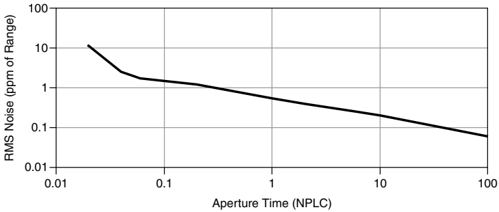
Figure 1. Noise Performance 2
