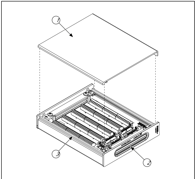
Figure 1. NI SCB-264X Shielded Connector Block
