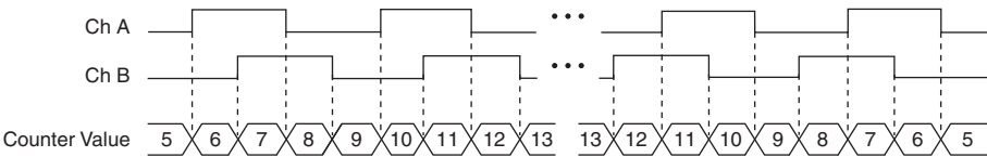
Figure 6-20. X4 Encoding
