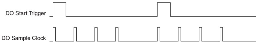
Figure 5-8. Retriggerable DO
