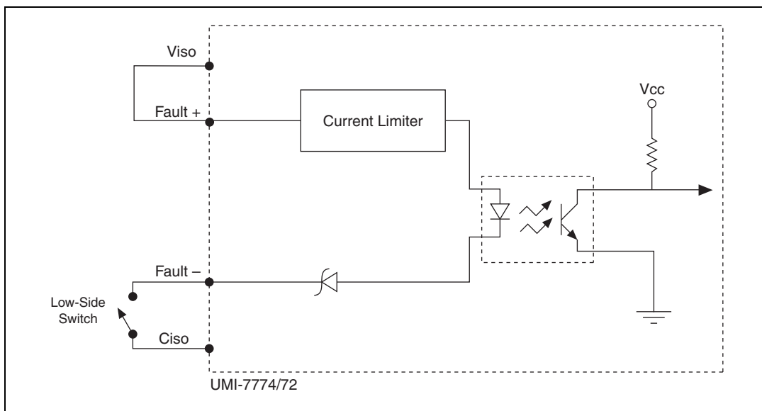
Figure 18. Example of Wiring a Low-Side Switch to the Fault Input
