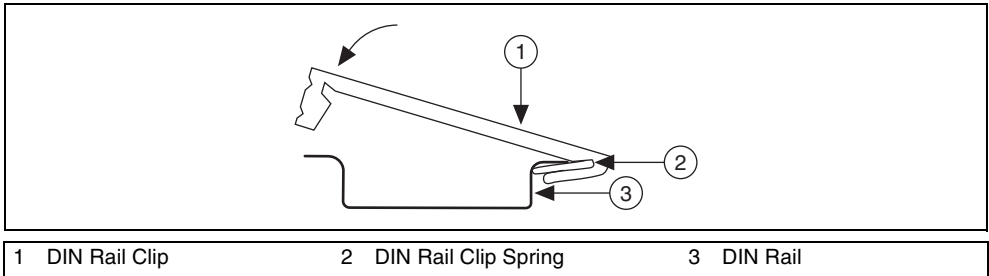
Figure 7. One Edge of DIN Rail Inserted in Clip
