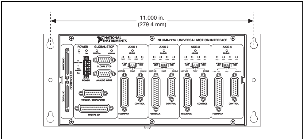
Figure 10. UMI-7774/72 Front View with Horizontal Panel Mount Dimensions
